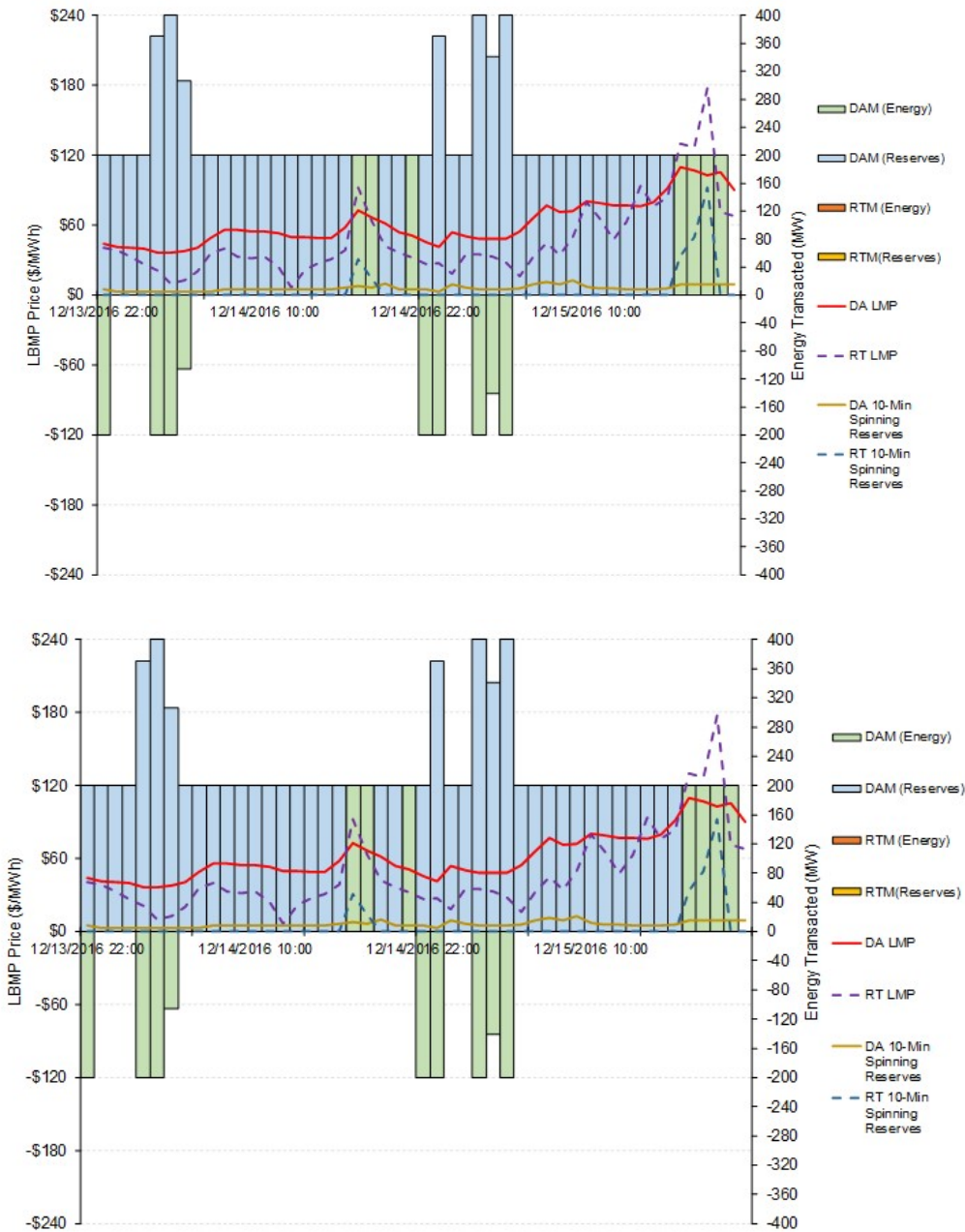
Figure 1: AGI Battery Model Step 1 Example: Zone G (Rockland), December 14-15, 2016, 4-Hour Battery
